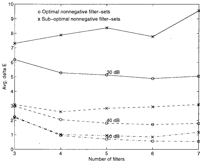
Fig. 1. Performance comparison of optimal and suboptimal filter sets.
